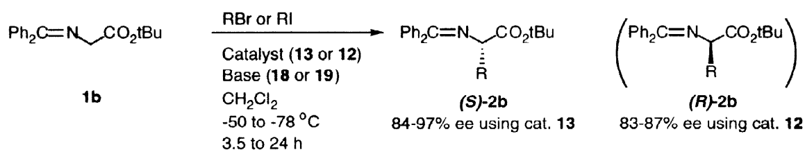
Scheme 10. Homogeneous Catalytic Enantioselective Synthesis of \alpha -Amino Acid Derivatives.
