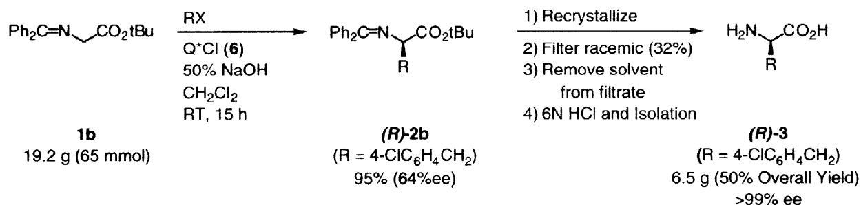
Scheme 5. “Large-Scale” Room-Temperature Synthesis of an Optically Pure Amino Acid by Chiral PTC.
