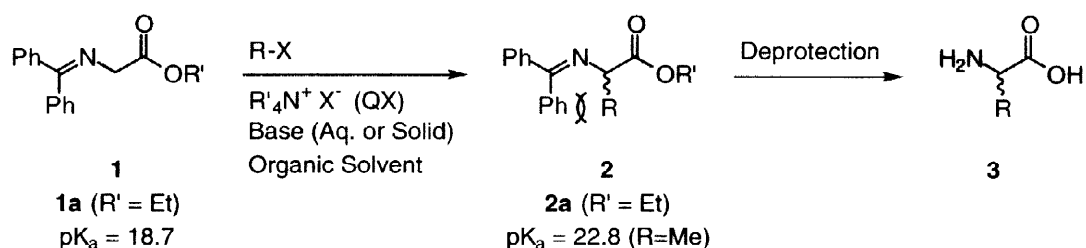
Scheme 1. Synthesis of \alpha -Amino Acids by Phase-Transfer Catalysis.
