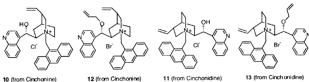
Scheme 3. Three Generations of Chiral, Non-Racemic PTC Catalysts Derived from the Cinchona Alkaloids.
