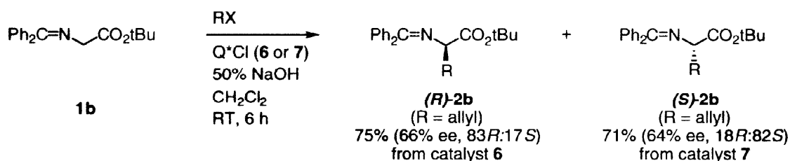
Scheme 4. Catalytic Enantioselective Synthesis of \alpha -Amino Acid Derivatives using “First Generation” PTC Catalysts.
