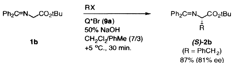
Scheme 6. Catalytic Enantioselective Synthesis of \alpha -Amino Acid Derivatives with “Second Generation” PTC Catalysts.
